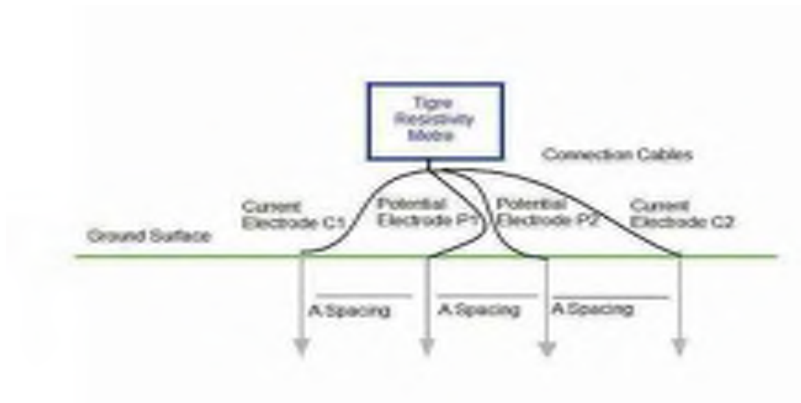
Figure 1: Resistivity Testing using the Wenner Array.
