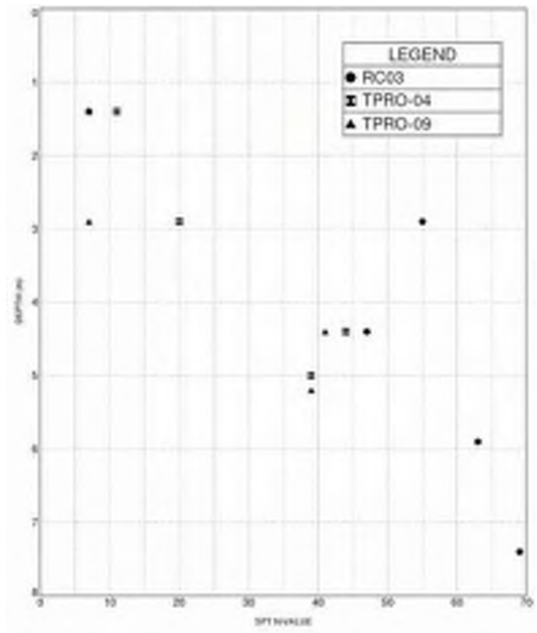
Figure 10 – SPT Vs Depth plot for TPRO-04, TPRO-09 & RC03
